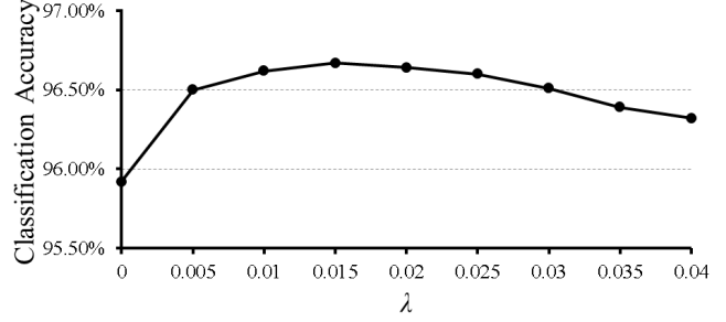
Figure 6. Comparison of face/non-face classification accuracy of models (without ICS) trained with different \lambda on validation set.
