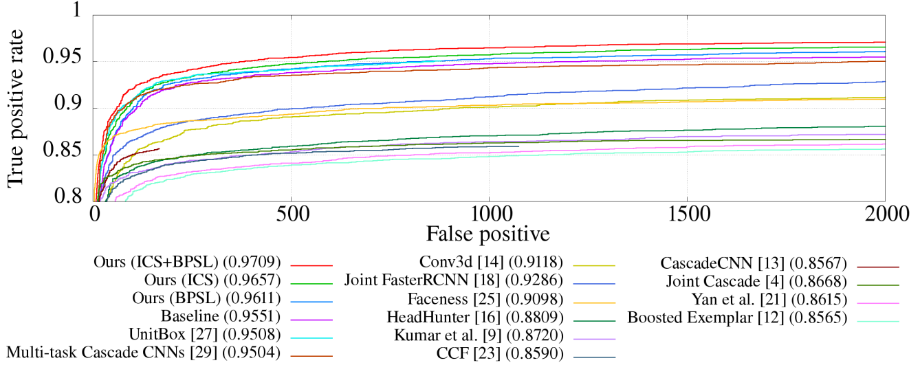
Figure 7. Receiver Operating Characteristic curves (ROC) obtained by our proposed method (with different proposed components) and other techniques on Fddb. ICS denotes inside the cascaded structure (i.e., ERC and DR layer). BPSL denotes body part sensitive learning (i.e., localize body part in training). ‘Baseline’ denotes neither use ICS nor BPSL. Best viewed in color.
